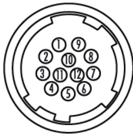
Hirose 12 Pin
